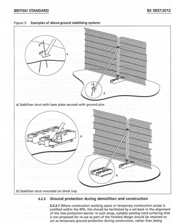
DETAIL 2 Fencing specification reproduced from BS 5837:2012 Trees in relation to design, demolition, and construction Recommendations.
