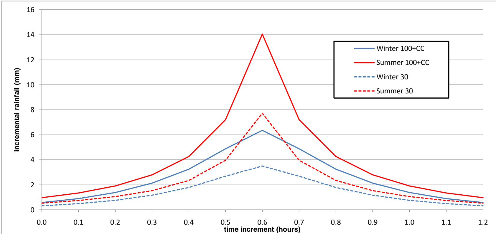
design storm profiles for Abermule from FEH CD-ROM DDF statistics
